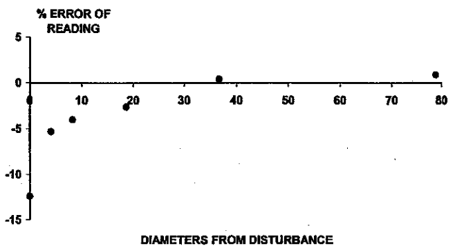
Fig. 13. Errors downstream of a gate valve 2/3 open.
