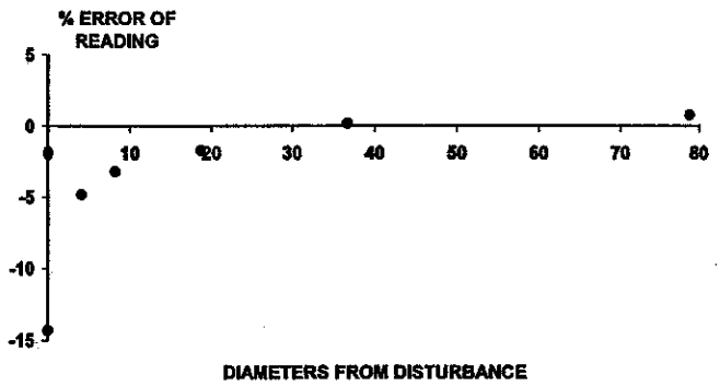
Fig. 12. Errors from a butterfly valve 1/3 open.
