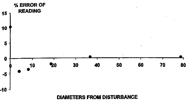
Fig. 6. Errors downstream of a conical contraction.
