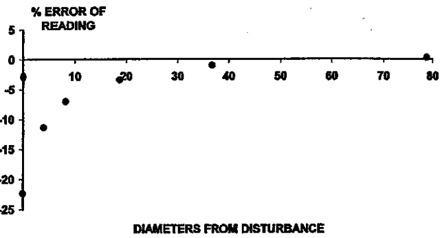
Fig. 8. Errors downstream of a single 90 degree bend.
