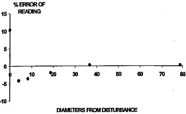
Fig. 7. Errors downstream of a conical expansion.
