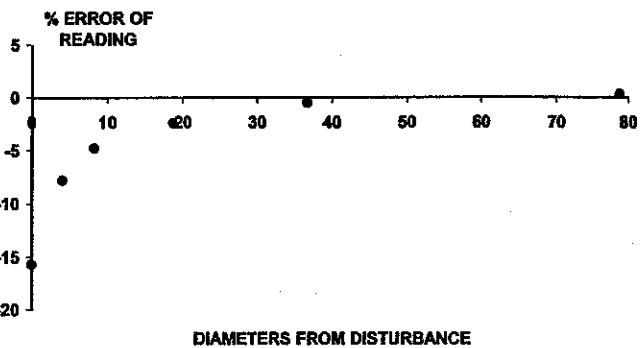
Fig. 9. Errors downstream of two 90 degree bends in 'U' configuration.
