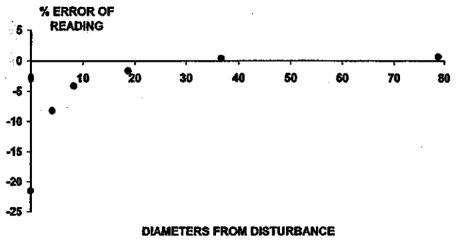
Fig. 11. Errors downstream of a butterfly valve 2/3 open.
