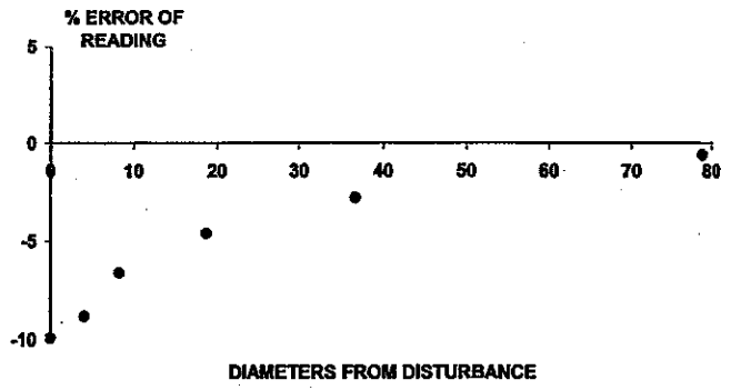
Fig. 10. Errors from two 90 degree bends in perpendicular planes.
